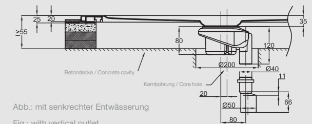
Fig.: with vertical outlet
